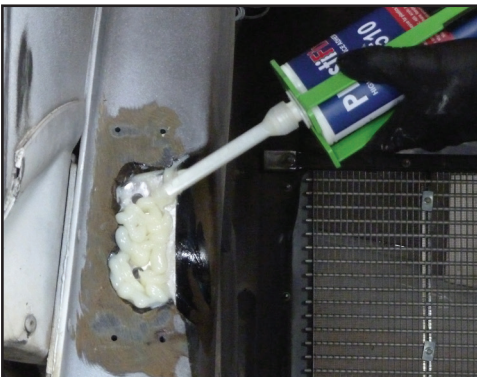
Fill the broken-out area on the side of the plug with adhesive, then coat the sanded side of the bearing plate with adhesive.
