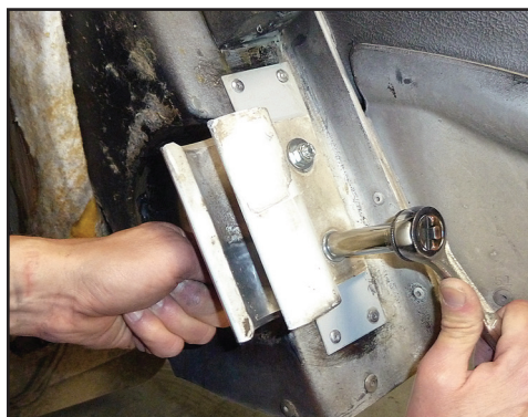
Install the hood brackets using the supplied 5/16" x 1-3/4" bolts, nuts, and washers. Use a flat washer under both the bolt head and lock nut.
