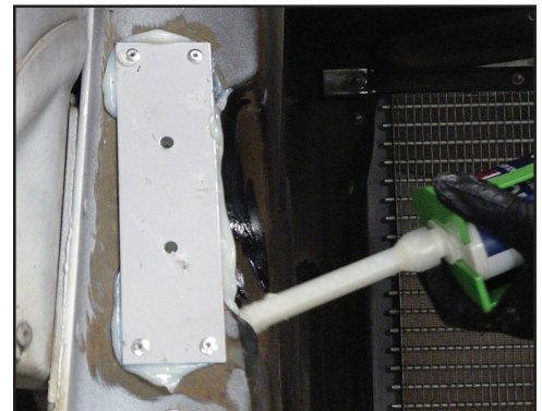
Fill the gap between the plate and the plug completely with PlastiFix. Clean up excess with a gloved finger or body spreader. Let cure for 2 to 4 hours minimum at 70°F. *
